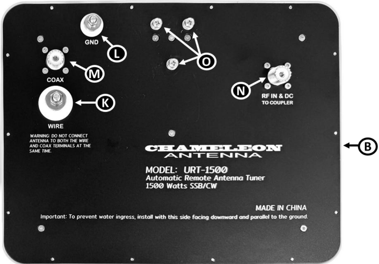
Plate 3. Tuner Unit.
