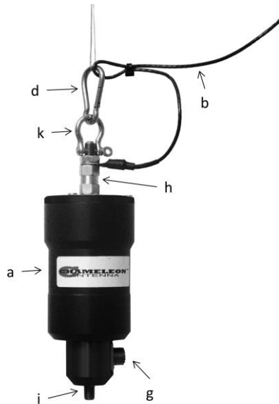
Plate 3. Hybrid Base Electrical and Mechanical Connections.
