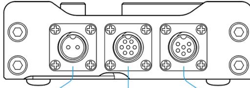
DC 9-15V Power supply
