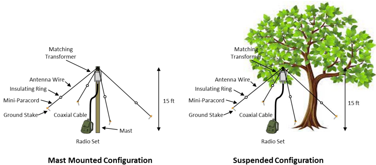
Figure 3. CHA NVIS Setup Options.
