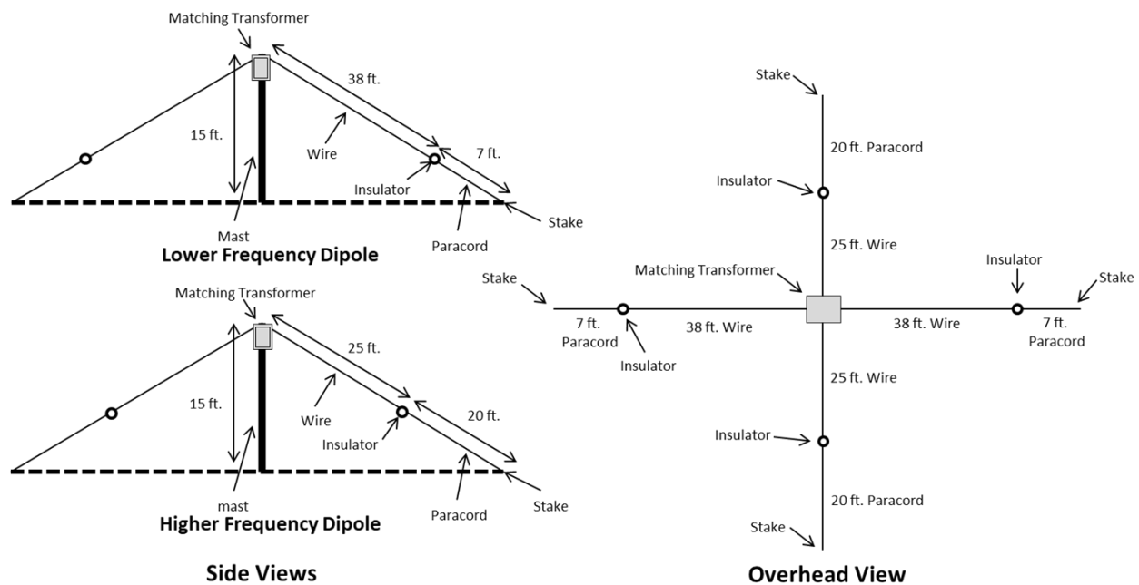
Figure 2. CHA NVIS Antenna Side and Overhead Views.
