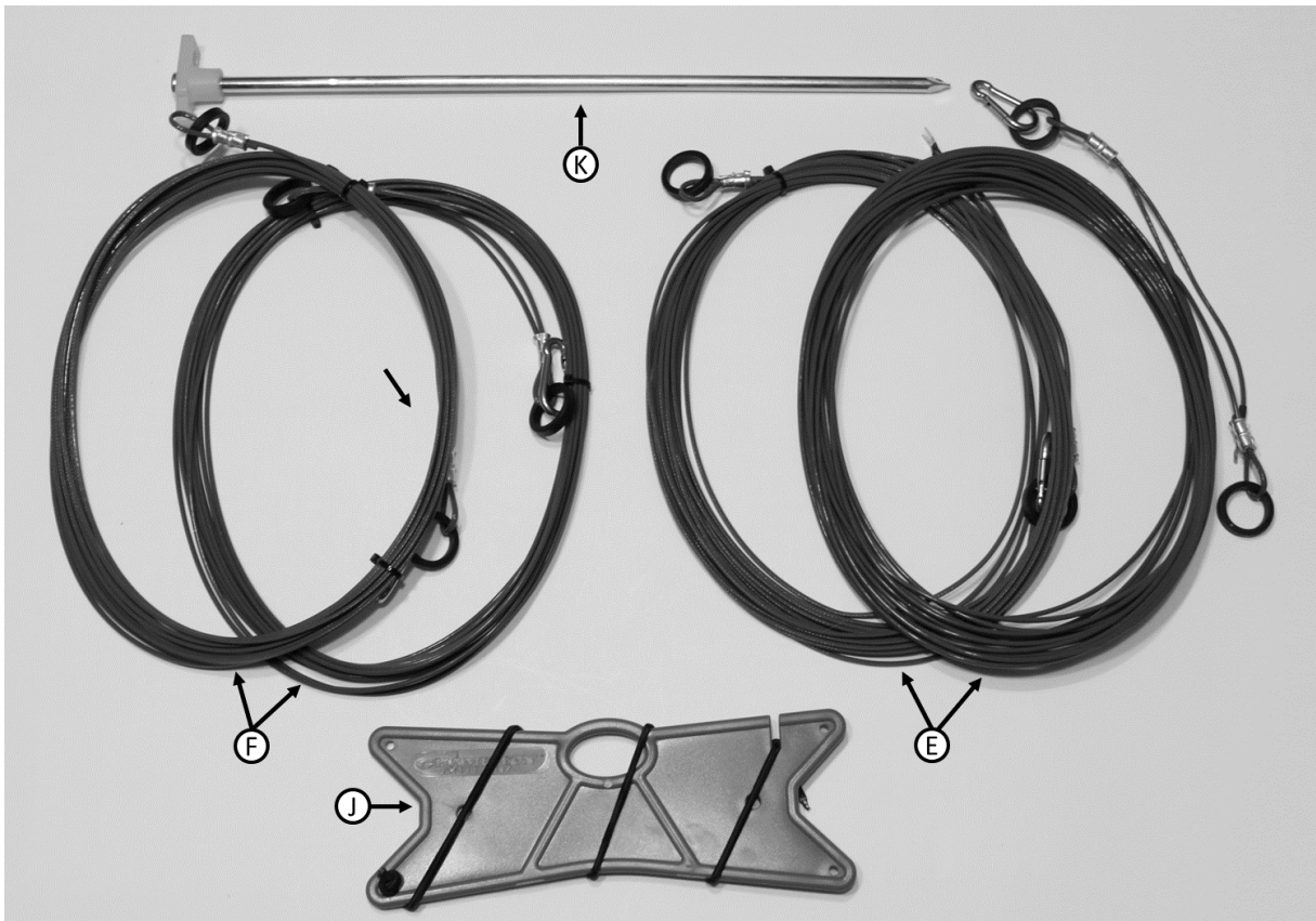
Plate 5. CHA NVIS Components.
